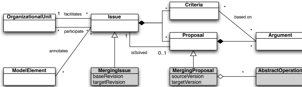
Figure 3. Merging Issue Model (UML class diagram)
