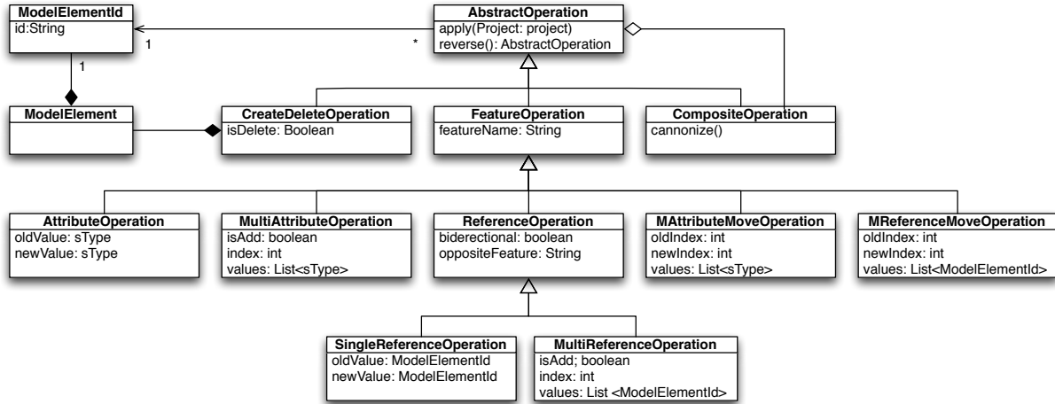
Figure 2. Operations Taxonomy (UML class diagram)
