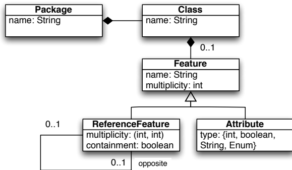
Figure 1. EMF Ecore (UML class diagram)
